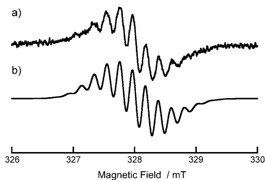
Figure 2. ESR spectra of 1^{\bullet+} : a) in \text{CH}_2\text{Cl}_2 at 233 K; b) simulated.
