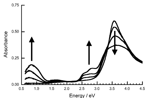
Figure 3. UV/Vis/NIR spectra of the stepwise electrochemical oxidation of 1 to 1^{2+} in \text{CH}_2\text{Cl}_2/0.1 \text{ M } n\text{Bu}_4\text{N}^+\text{BF}_4^- at room temperature.
